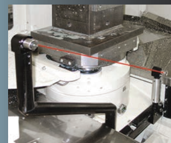
Spindle and Tool Probes
