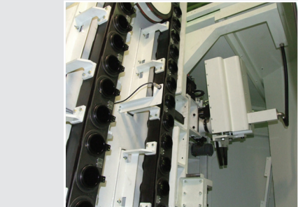
Sub Arm feeds tool to swing pot.
