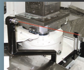
Spindle and Tool Probes
