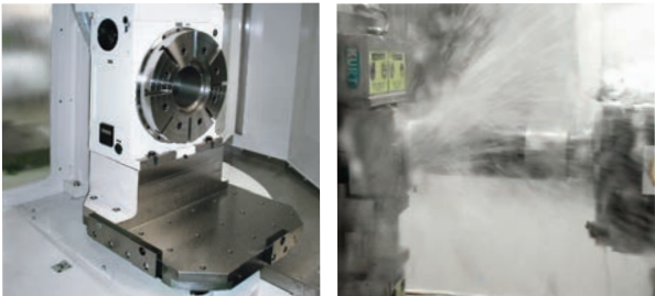
Field Retrofitable 5th Axis Rotary Tables (available on both pallets) Up to 1000psi Coolant Thru the Spindle Available
